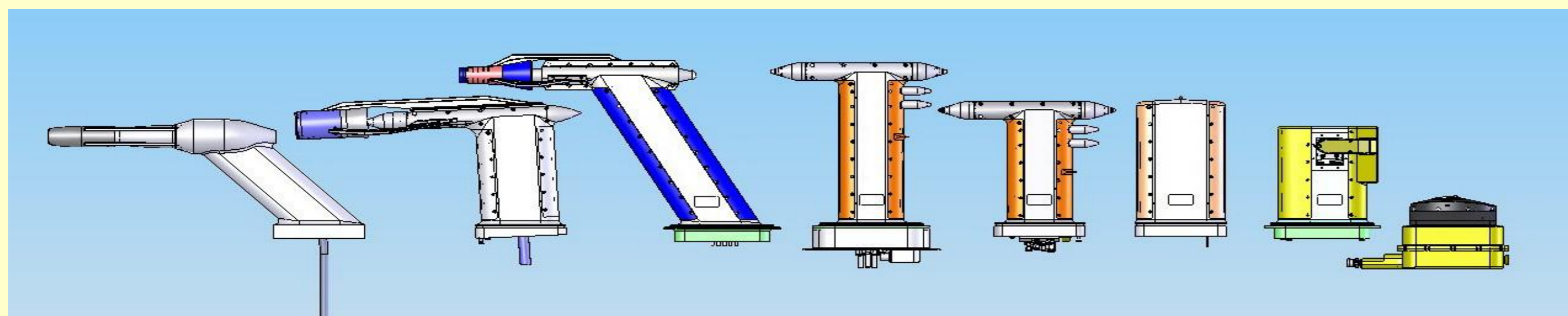
Variety of different inlets for HALO currently under development at enviscope : MAI, CVI, HASI, TGI-430, TGI-320, DUALER, HAI, SPARM
